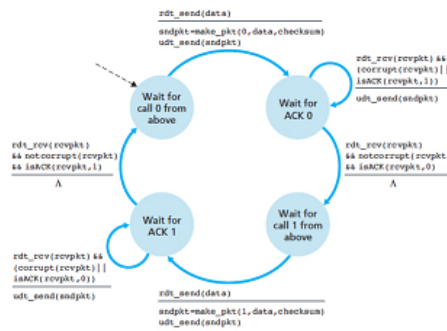
Figure 3.13 • rdt.2 sender
