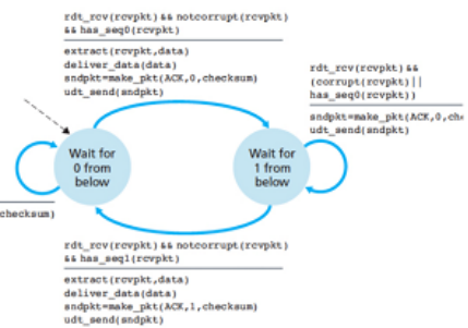
Figure 3.14 • rdt.2 receiver
